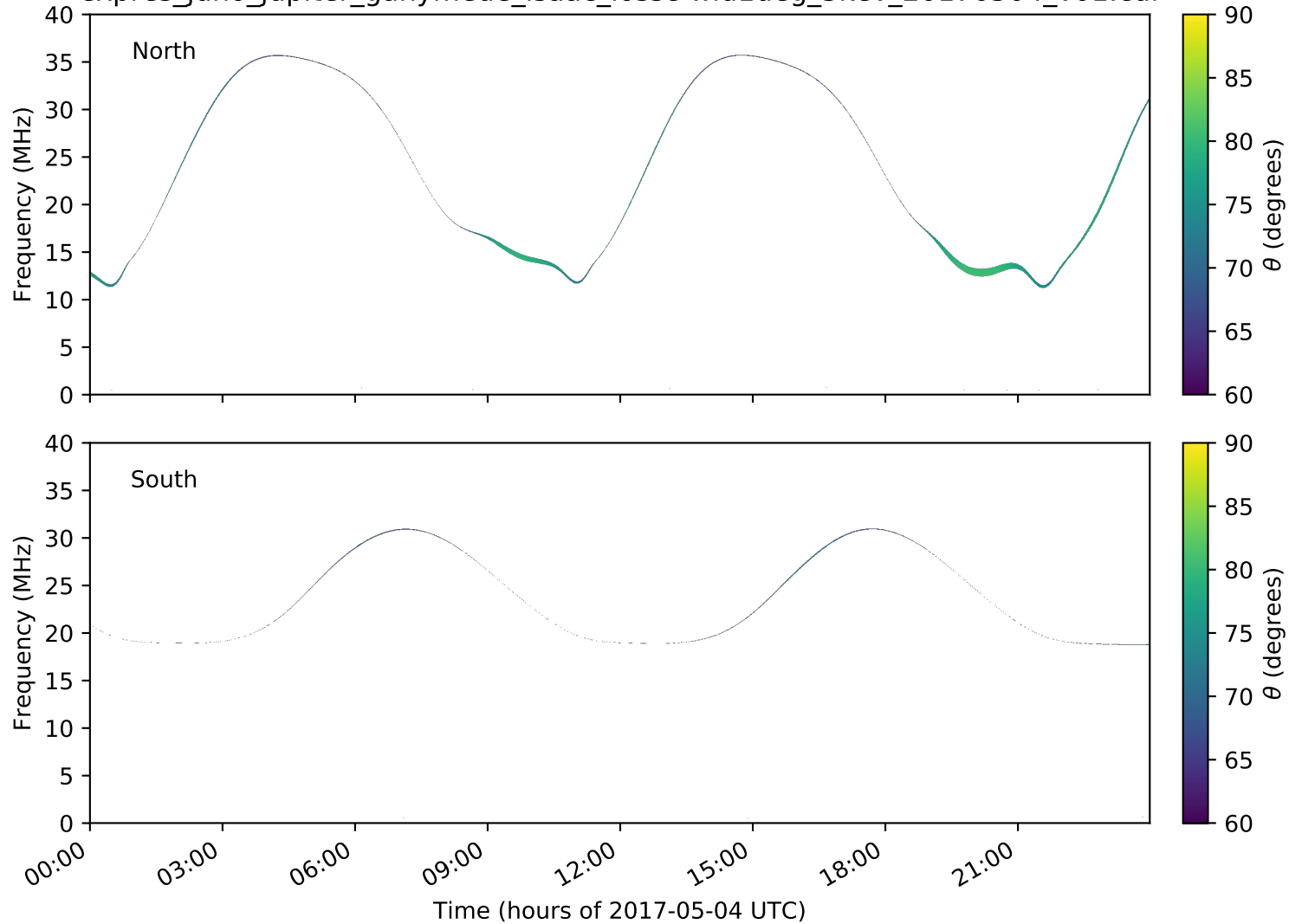
expres_juno_jupiter_ganymede_isaac_lossc-wid1deg_3kev_20170504_v01.cdf
