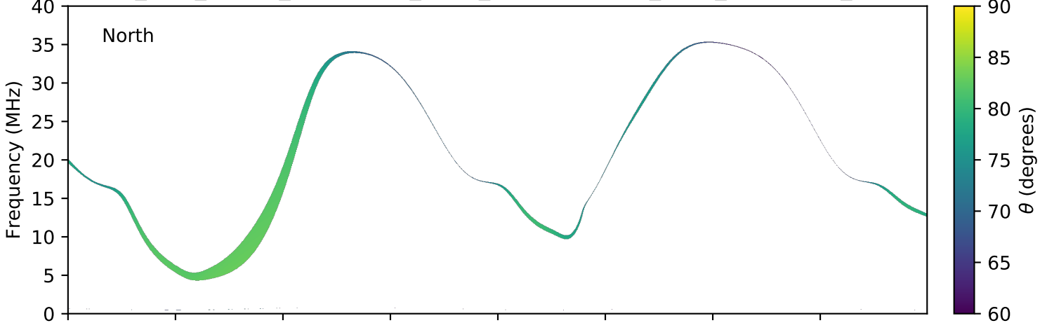
expres_juno_jupiter_ganymede_isaac_lossc-wid1deg_3kev_20170503_v01.cdf
