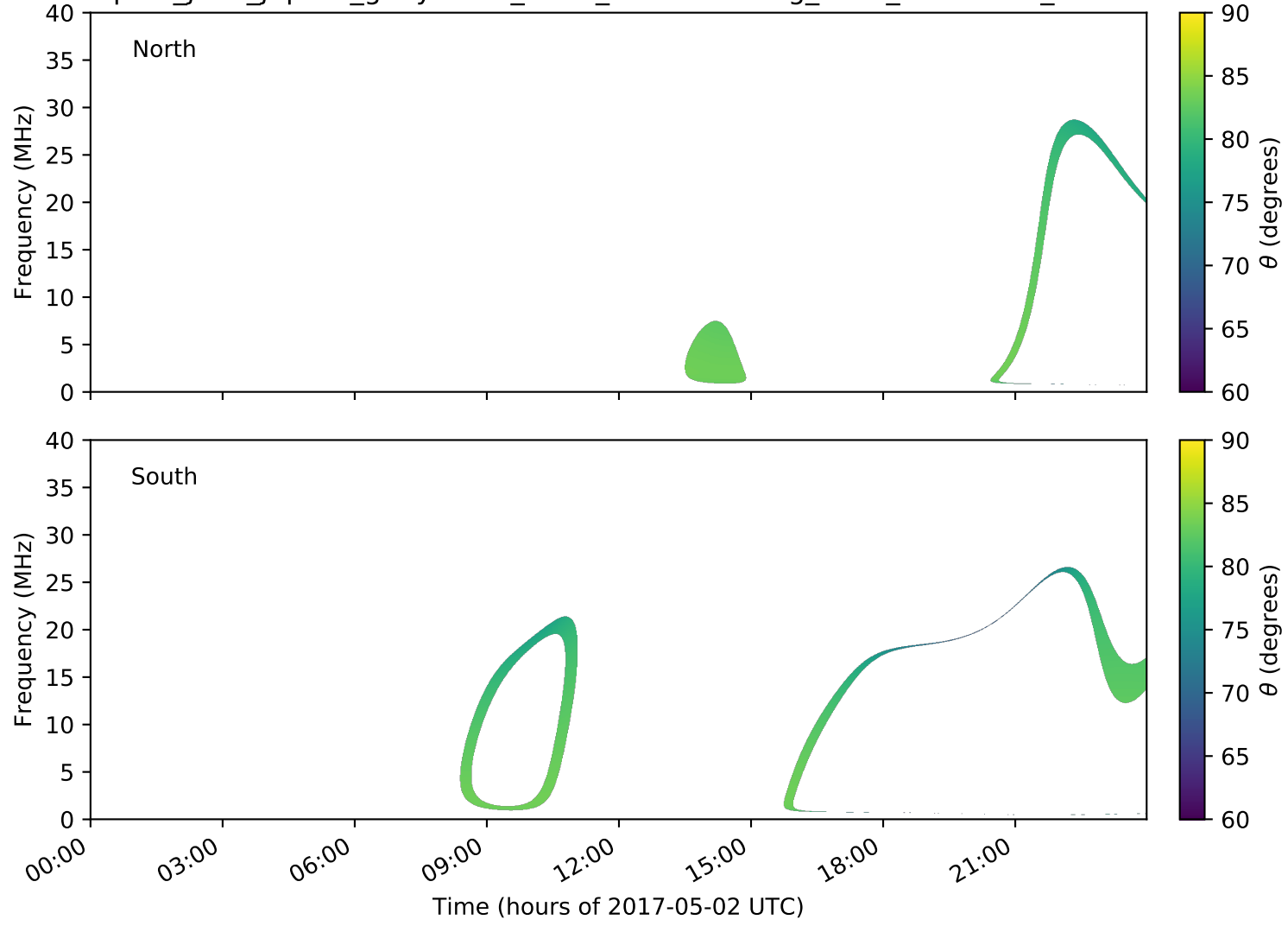
expres_juno_jupiter_ganymede_isaac_lossc-wid1deg_3kev_20170502_v01.cdf
