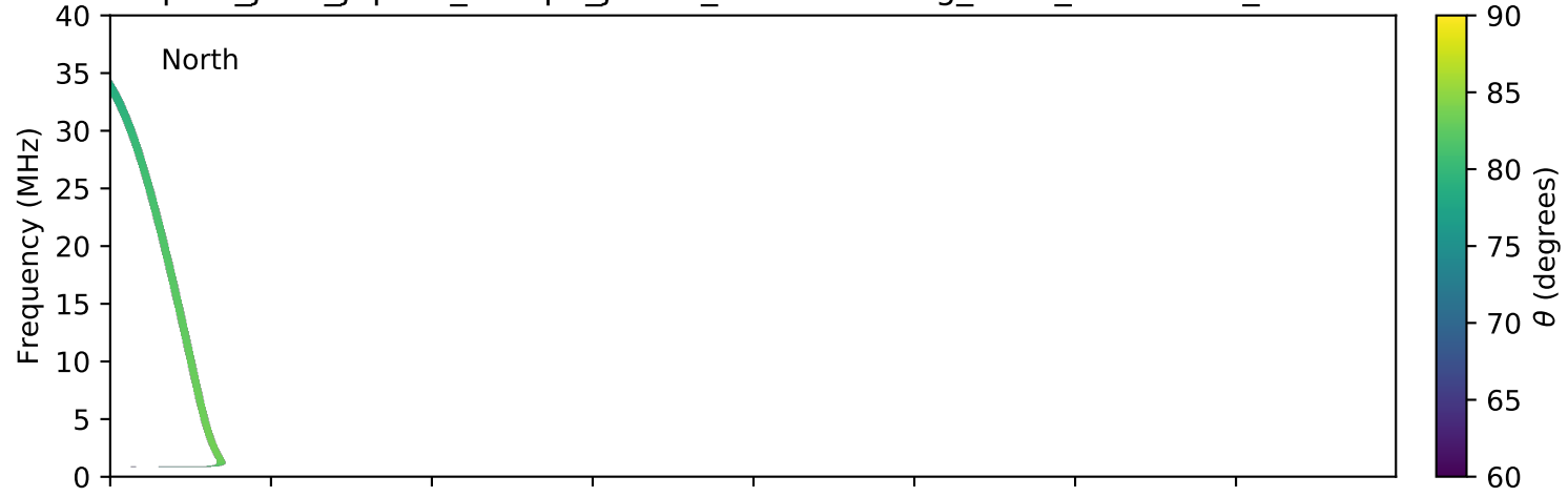
expres_juno_jupiter_europa_jrm09_lossc-wid1deg_3kev_20170508_v01.cdf
