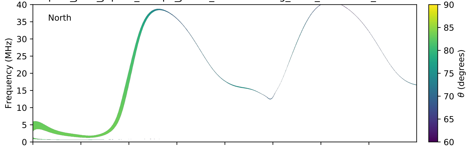
expres_juno_jupiter_europa_jrm09_lossc-wid1deg_3kev_20170503_v01.cdf
