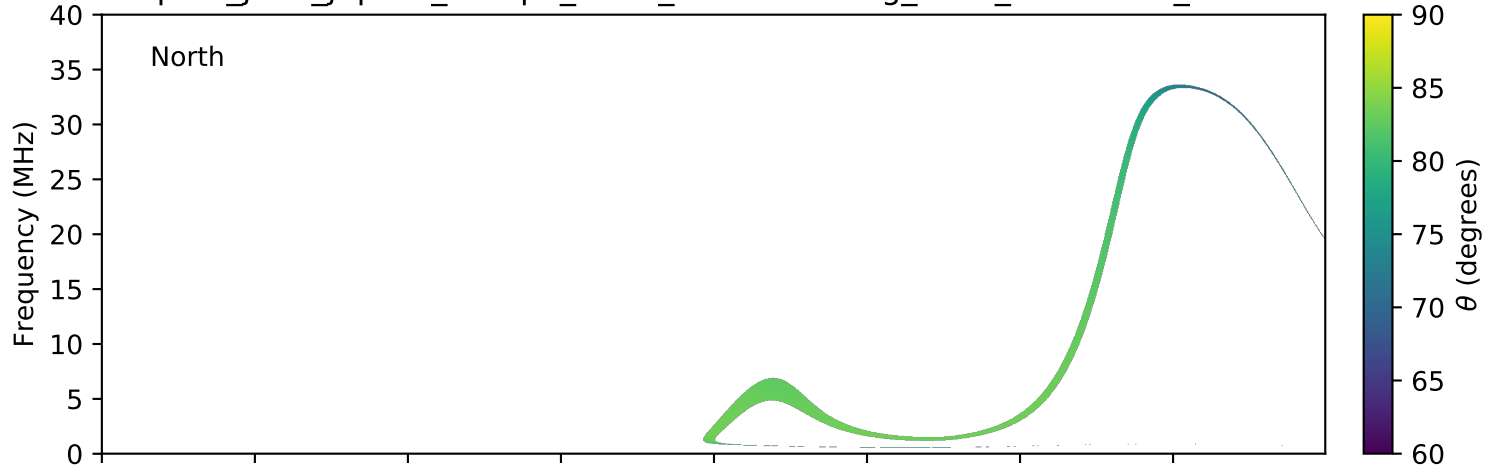
expres_juno_jupiter_europa_isaac_lossc-wid1deg_3kev_20170531_v01.cdf
