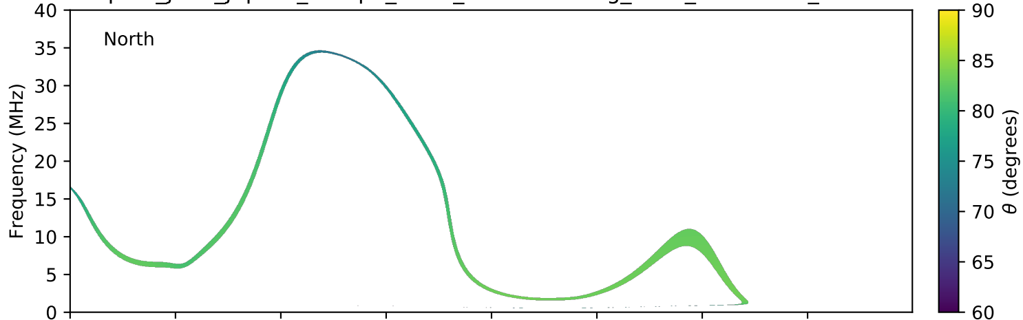
expres_juno_jupiter_europa_isaac_lossc-wid1deg_3kev_20170525_v01.cdf
