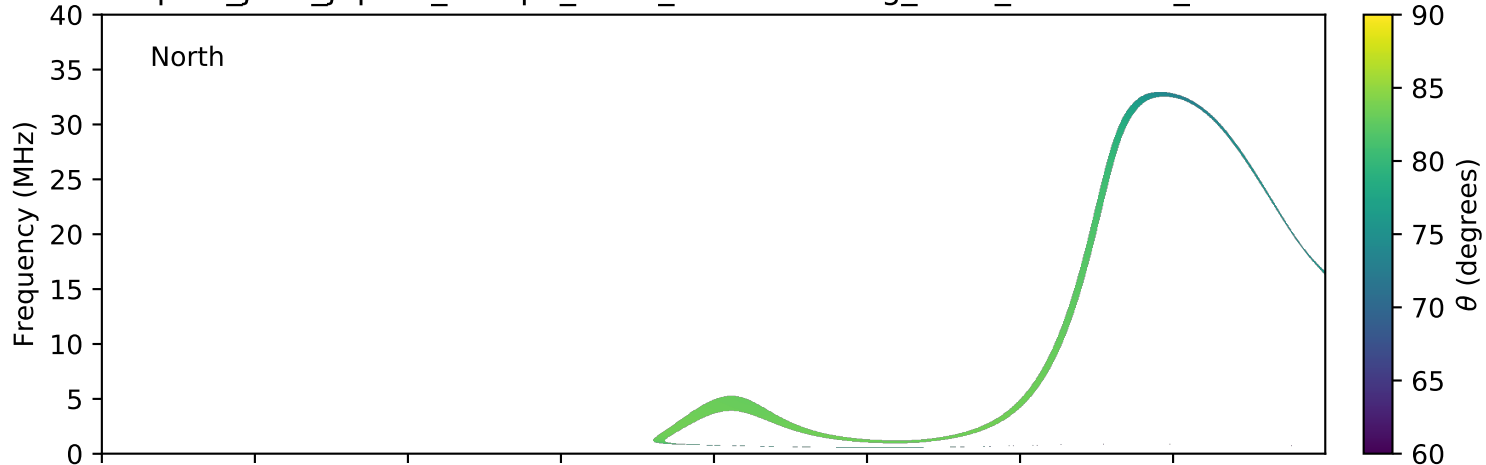
expres_juno_jupiter_europa_isaac_lossc-wid1deg_3kev_20170524_v01.cdf
