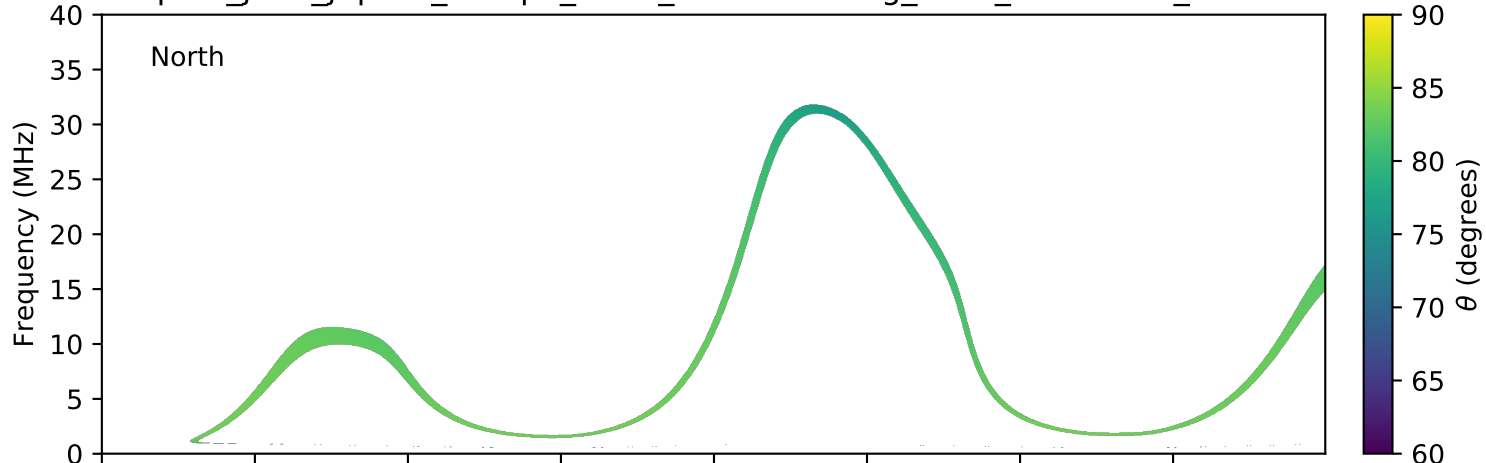
expres_juno_jupiter_europa_isaac_lossc-wid1deg_3kev_20170521_v01.cdf
