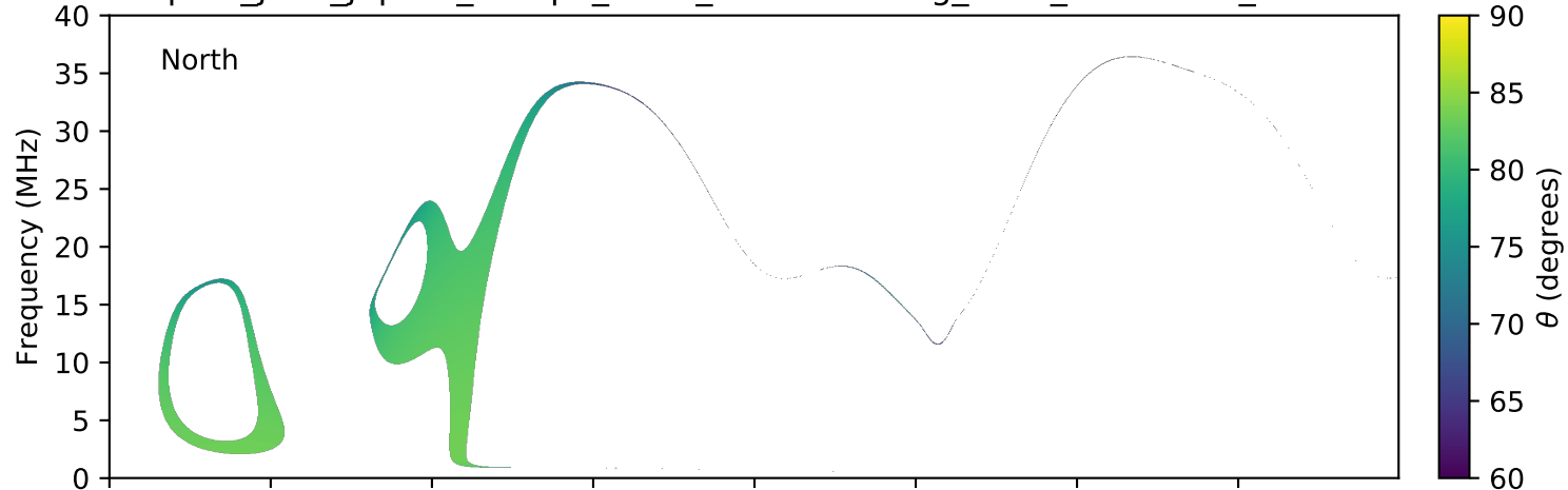
expres_juno_jupiter_europa_isaac_lossc-wid1deg_3kev_20170517_v01.cdf
