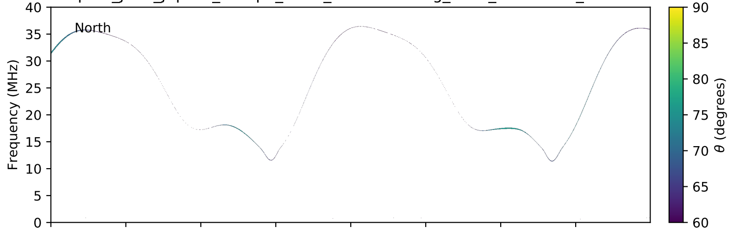
expres_juno_jupiter_europa_isaac_lossc-wid1deg_3kev_20170514_v01.cdf
