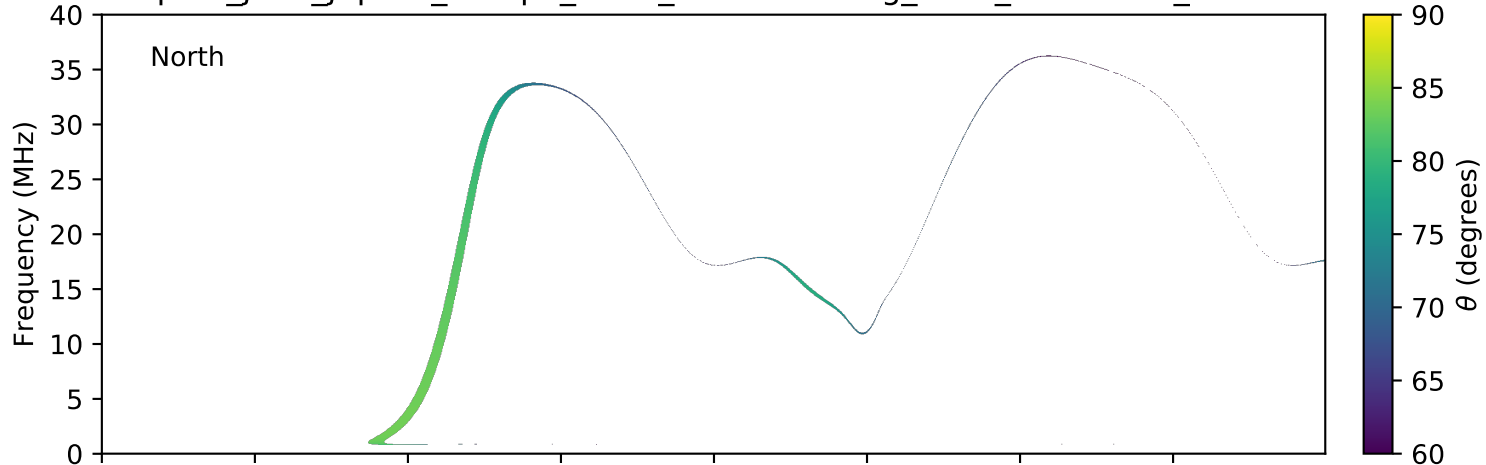
expres_juno_jupiter_europa_isaac_lossc-wid1deg_3kev_20170510_v01.cdf
