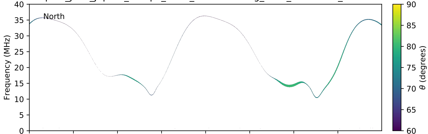
expres_juno_jupiter_europa_isaac_lossc-wid1deg_3kev_20170507_v01.cdf
