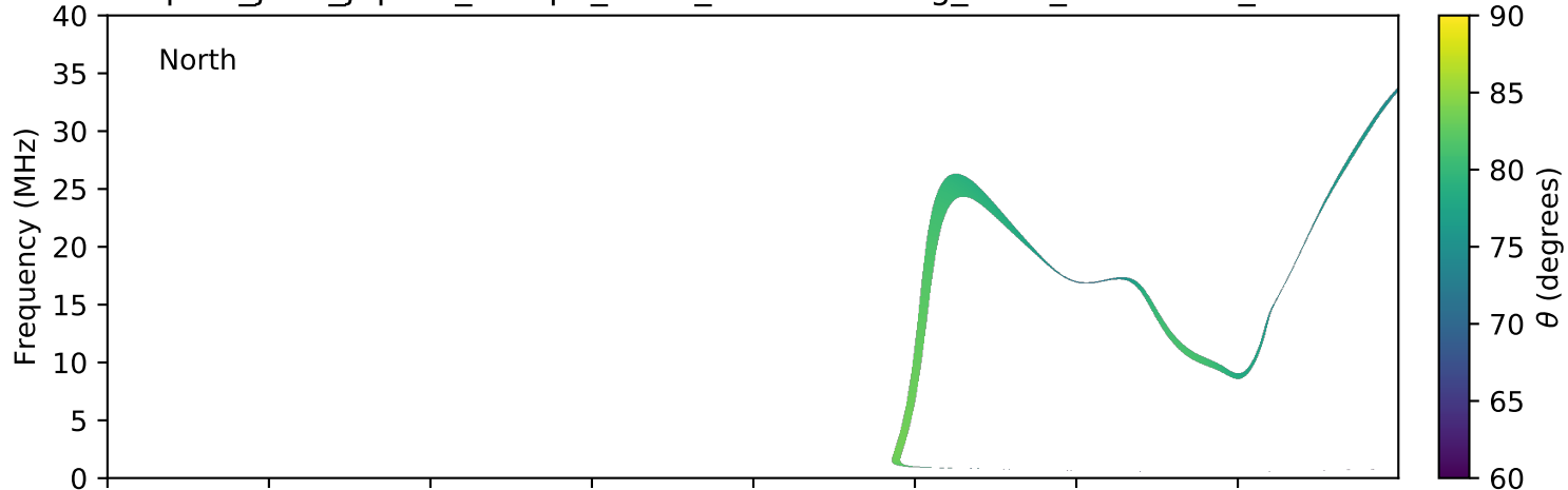
expres_juno_jupiter_europa_isaac_lossc-wid1deg_3kev_20170506_v01.cdf
