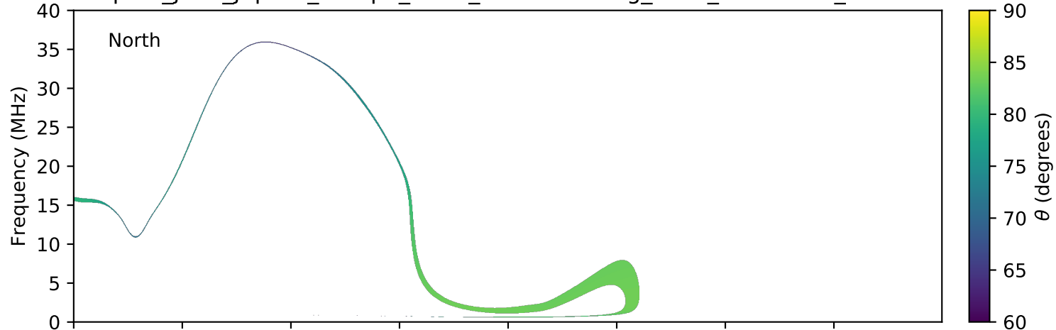
expres_juno_jupiter_europa_isaac_lossc-wid1deg_3kev_20170504_v01.cdf
