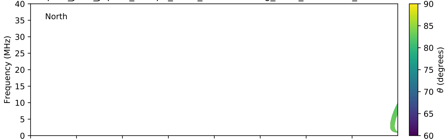
expres_juno_jupiter_europa_isaac_lossc-wid1deg_3kev_20170502_v01.cdf
