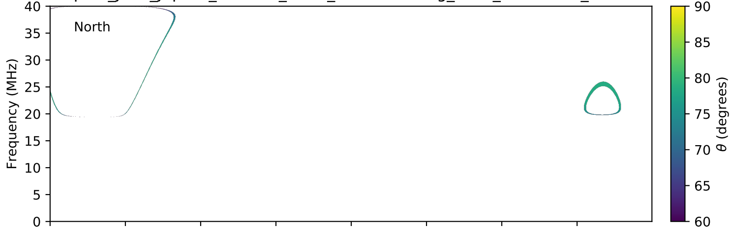
expres_juno_jupiter_174d-0r_isaac_lossc-wid1deg_9kev_20170519_v01.cdf
