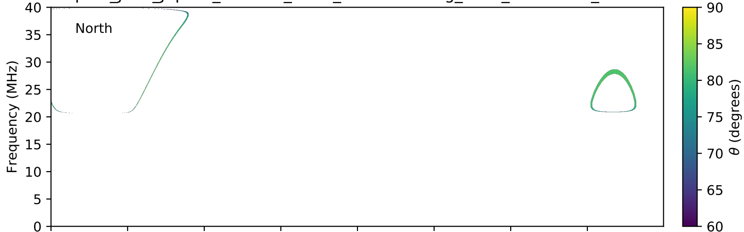
expres_juno_jupiter_174d-0r_isaac_lossc-wid1deg_5kev_20170519_v01.cdf
