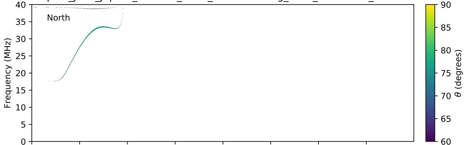
expres_juno_jupiter_106d-0r_isaac_lossc-wid1deg_9kev_20170519_v01.cdf
