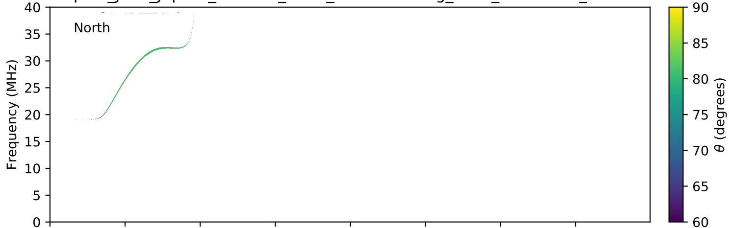
expres_juno_jupiter_106d-0r_isaac_lossc-wid1deg_5kev_20170519_v01.cdf
