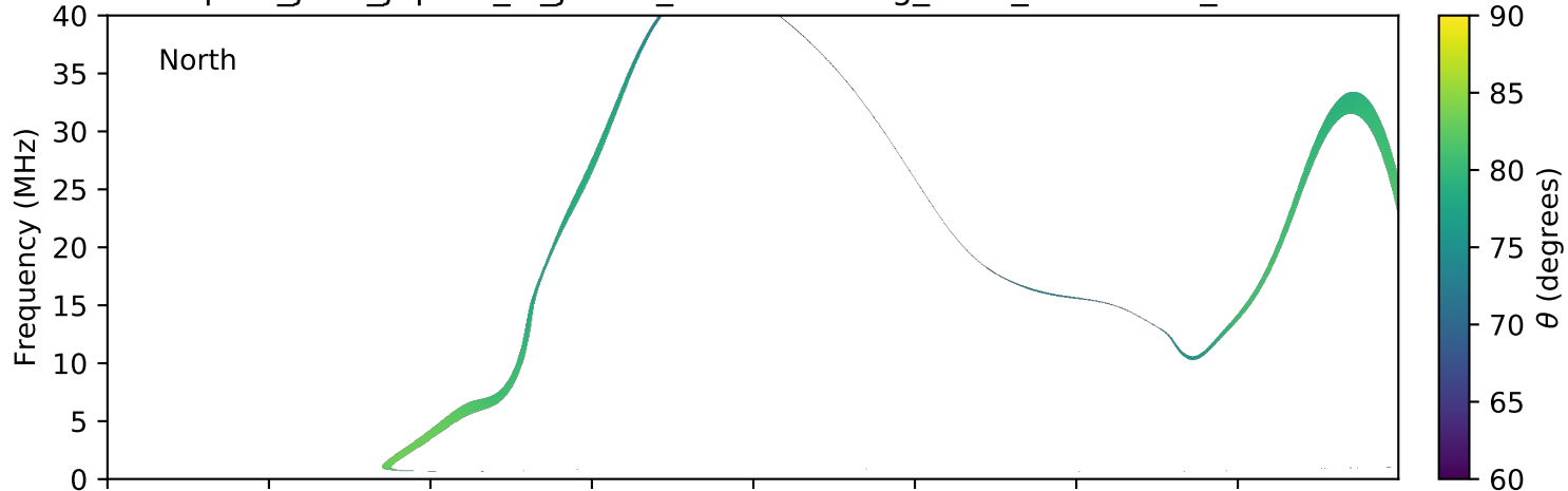
expres_juno_jupiter_io_jrm09_lossc-wid1deg_3kev_20170425_v01.cdf
