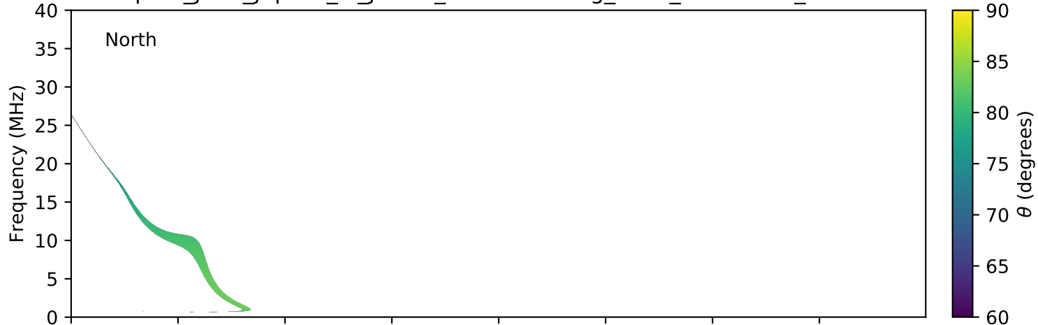
expres_juno_jupiter_io_jrm09_lossc-wid1deg_3kev_20170424_v01.cdf
