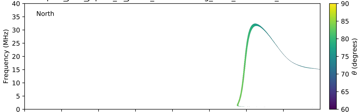
expres_juno_jupiter_io_jrm09_lossc-wid1deg_3kev_20170421_v01.cdf
