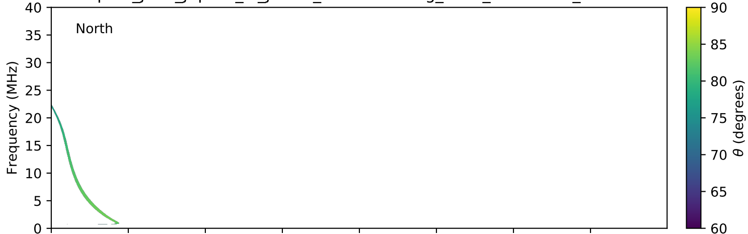
expres_juno_jupiter_io_jrm09_lossc-wid1deg_3kev_20170417_v01.cdf
