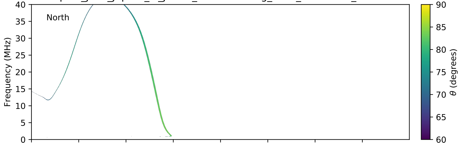
expres_juno_jupiter_io_jrm09_lossc-wid1deg_3kev_20170415_v01.cdf
