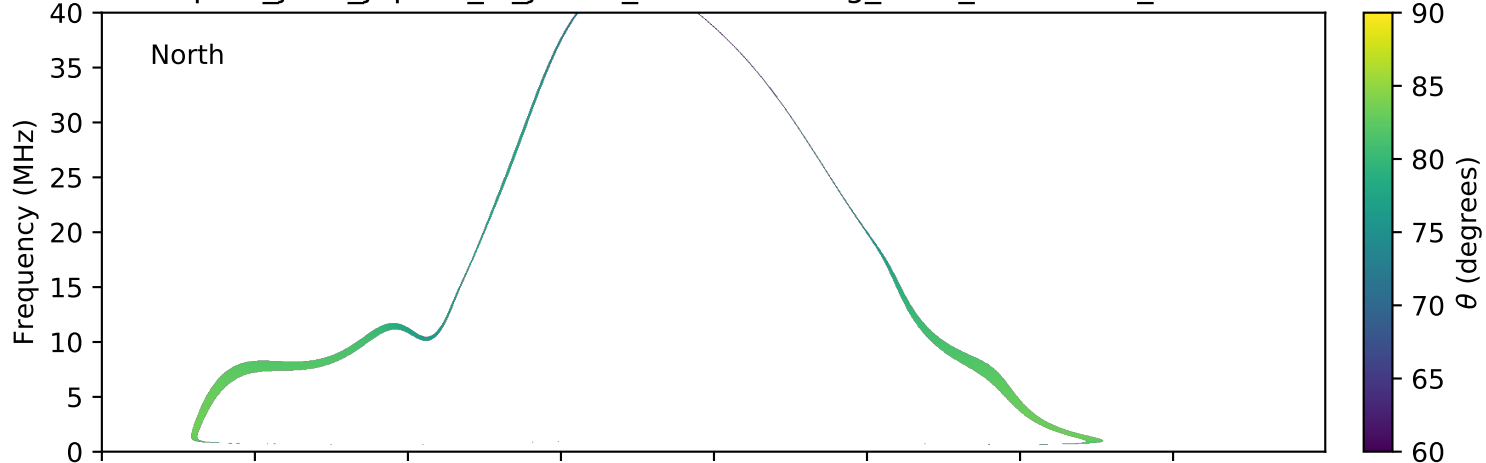
expres_juno_jupiter_io_jrm09_lossc-wid1deg_3kev_20170411_v01.cdf
