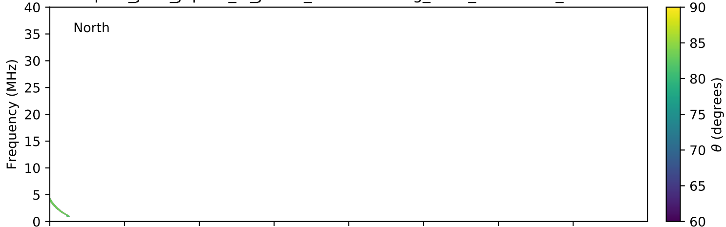
expres_juno_jupiter_io_jrm09_lossc-wid1deg_3kev_20170410_v01.cdf
