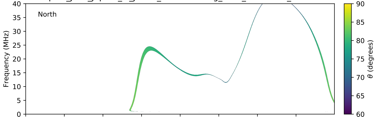
expres_juno_jupiter_io_jrm09_lossc-wid1deg_3kev_20170409_v01.cdf
