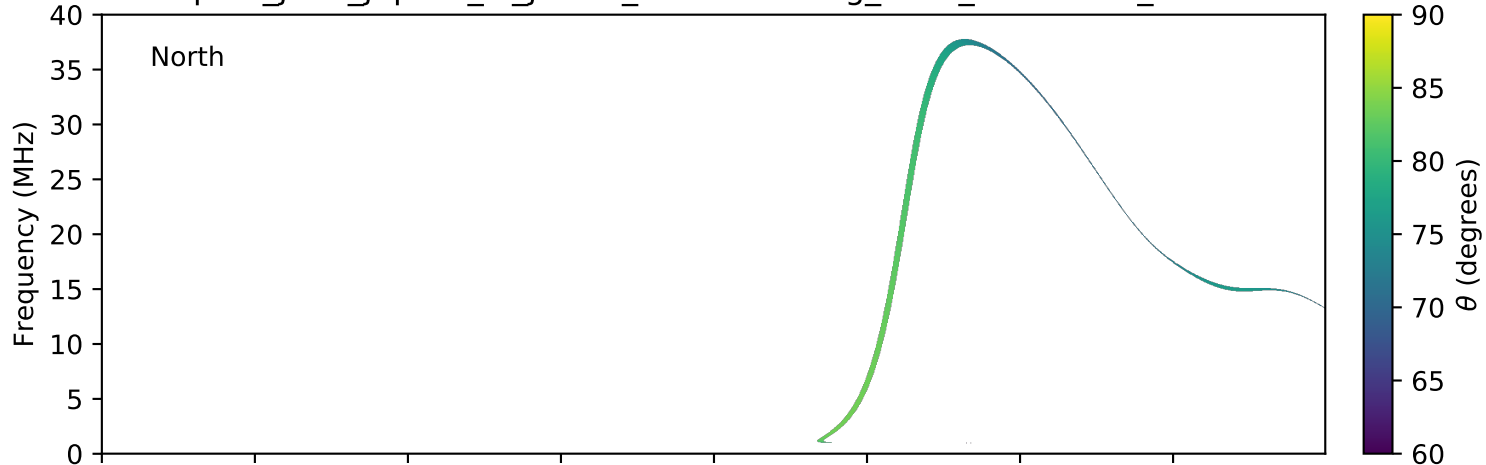
expres_juno_jupiter_io_jrm09_lossc-wid1deg_3kev_20170407_v01.cdf
