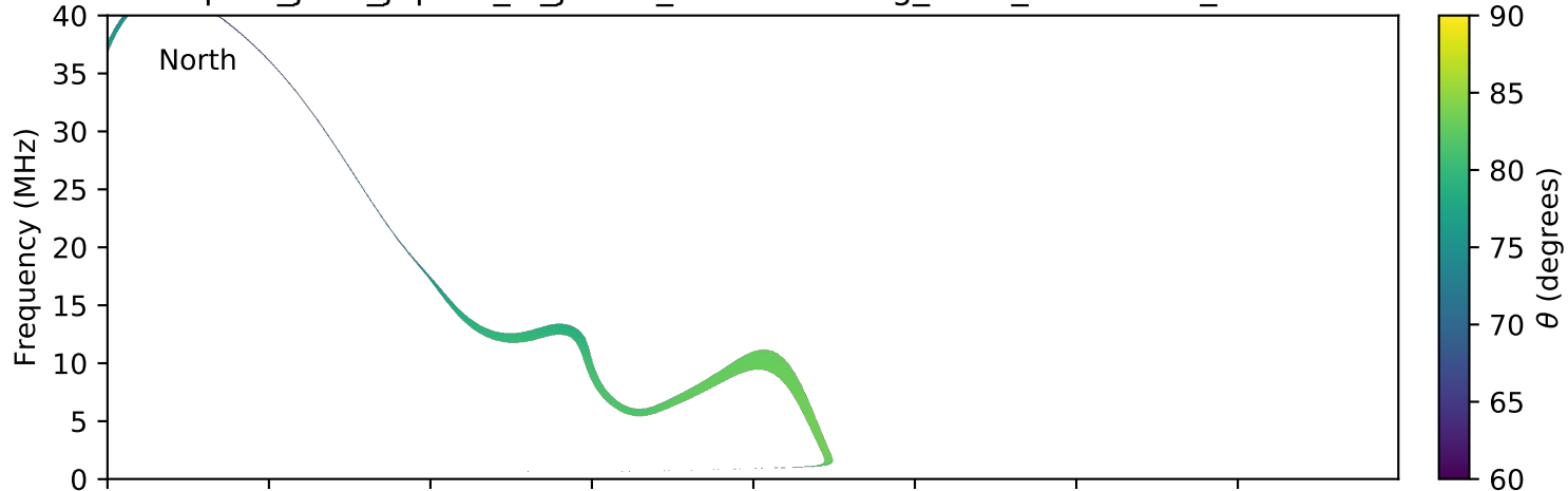
expres_juno_jupiter_io_jrm09_lossc-wid1deg_3kev_20170406_v01.cdf
