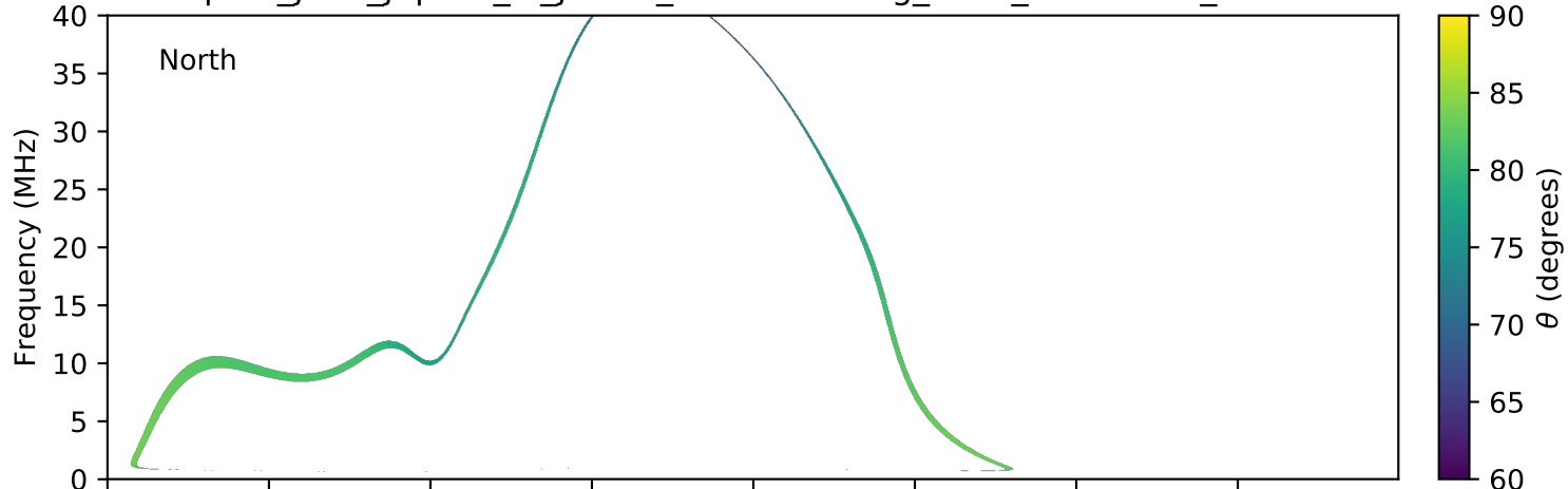
expres_juno_jupiter_io_jrm09_lossc-wid1deg_3kev_20170404_v01.cdf
