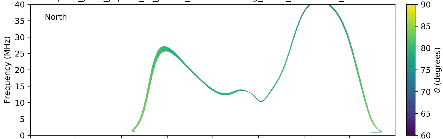
expres_juno_jupiter_io_jrm09_lossc-wid1deg_3kev_20170402_v01.cdf
