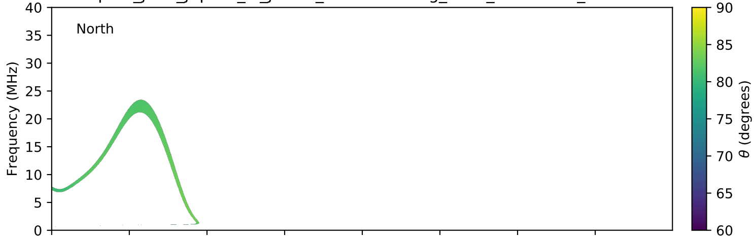
expres_juno_jupiter_io_jrm09_lossc-wid1deg_3kev_20170401_v01.cdf
