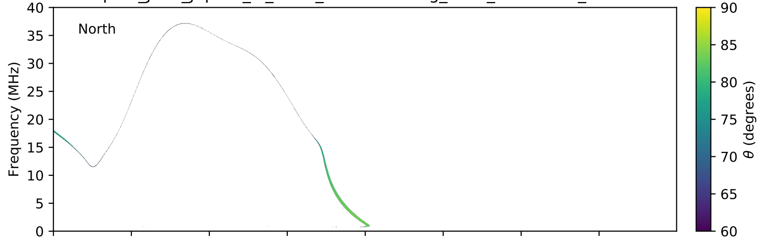
expres_juno_jupiter_io_isaac_lossc-wid1deg_3kev_20170429_v01.cdf
