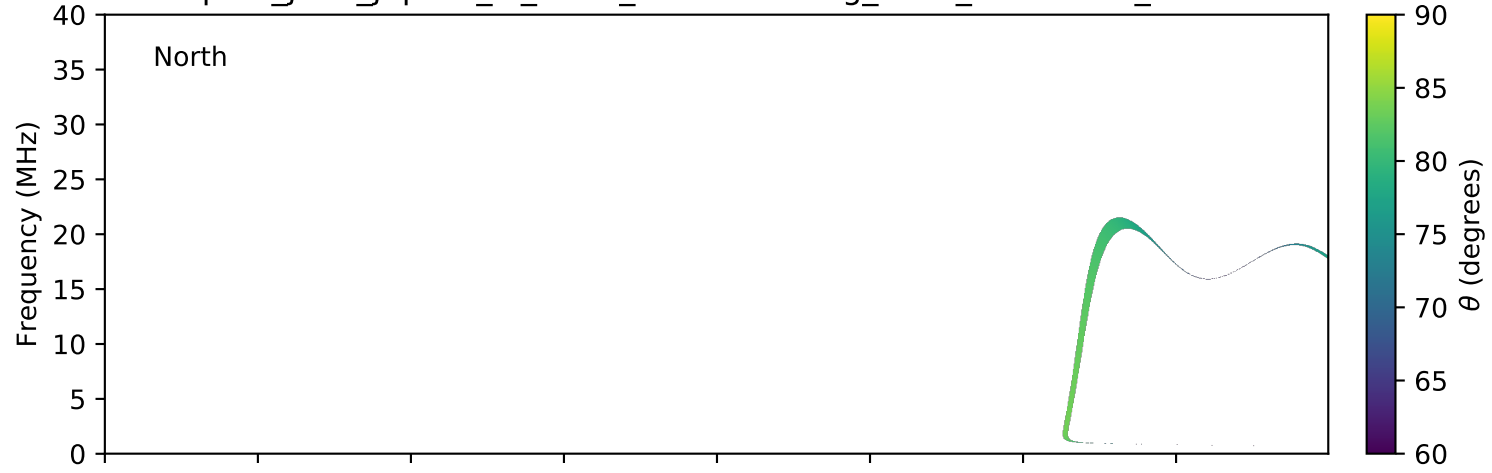
expres_juno_jupiter_io_isaac_lossc-wid1deg_3kev_20170428_v01.cdf
