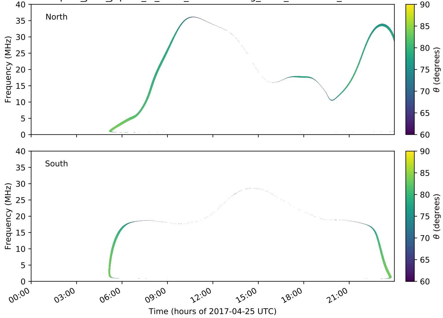
expres_juno_jupiter_io_isaac_lossc-wid1deg_3kev_20170425_v01.cdf
