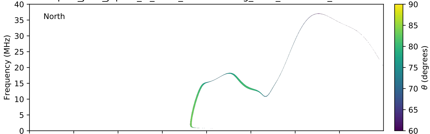
expres_juno_jupiter_io_isaac_lossc-wid1deg_3kev_20170423_v01.cdf
