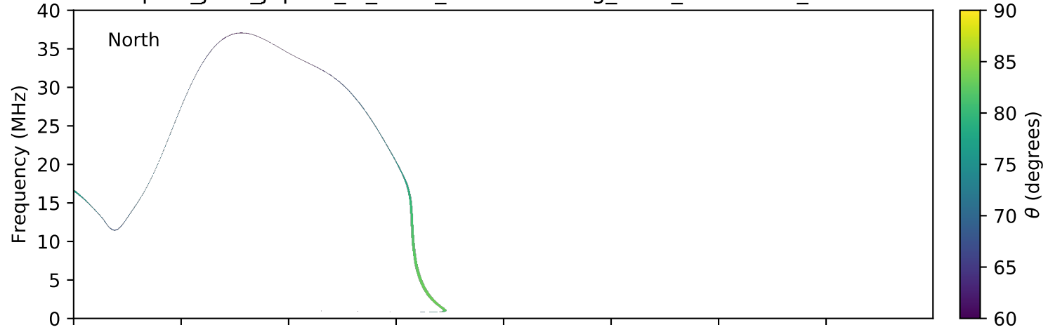
expres_juno_jupiter_io_isaac_lossc-wid1deg_3kev_20170422_v01.cdf
