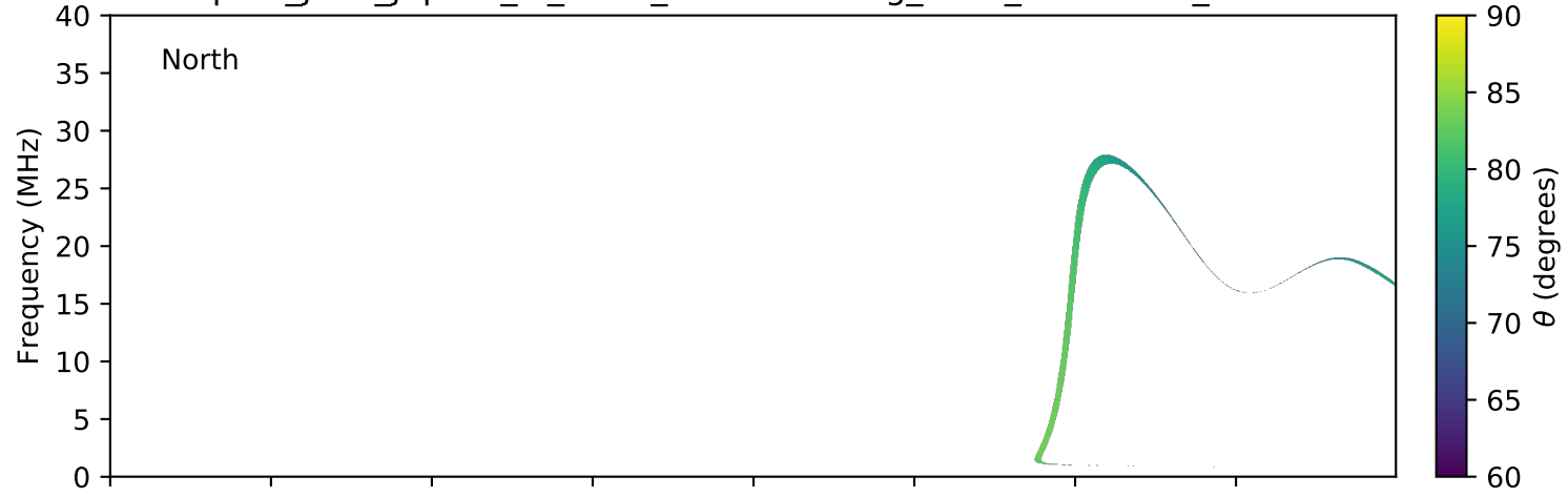
expres_juno_jupiter_io_isaac_lossc-wid1deg_3kev_20170421_v01.cdf
