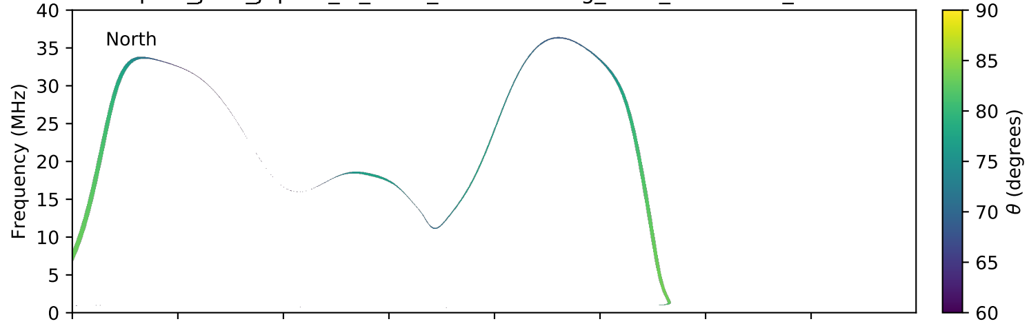
expres_juno_jupiter_io_isaac_lossc-wid1deg_3kev_20170420_v01.cdf
