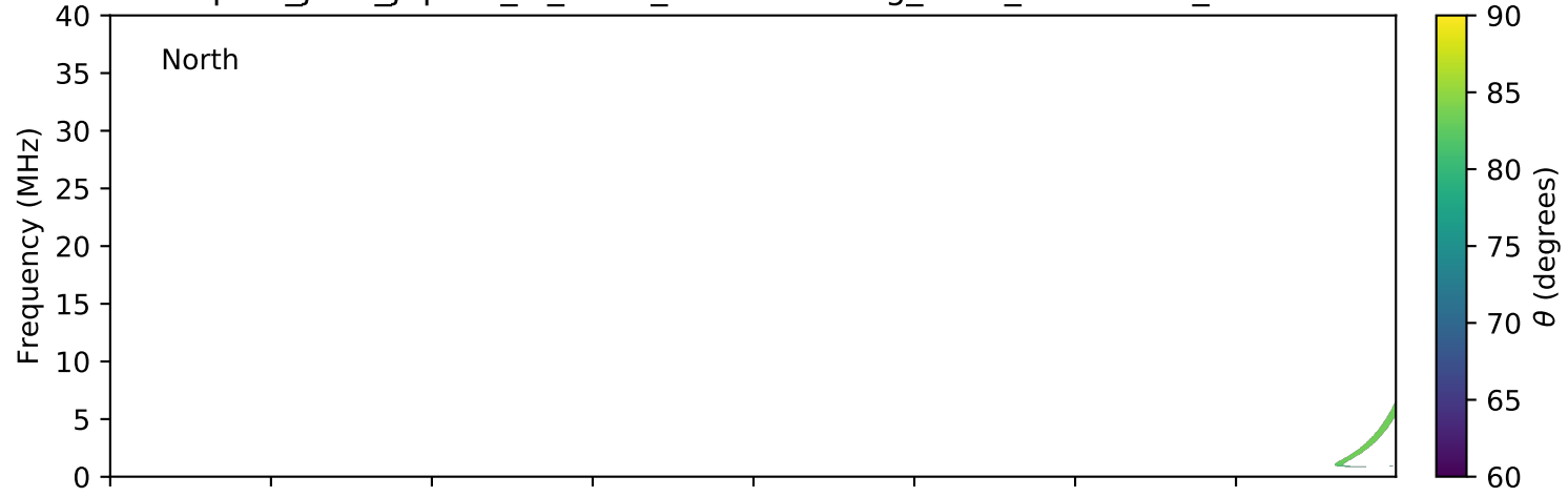
expres_juno_jupiter_io_isaac_lossc-wid1deg_3kev_20170419_v01.cdf
