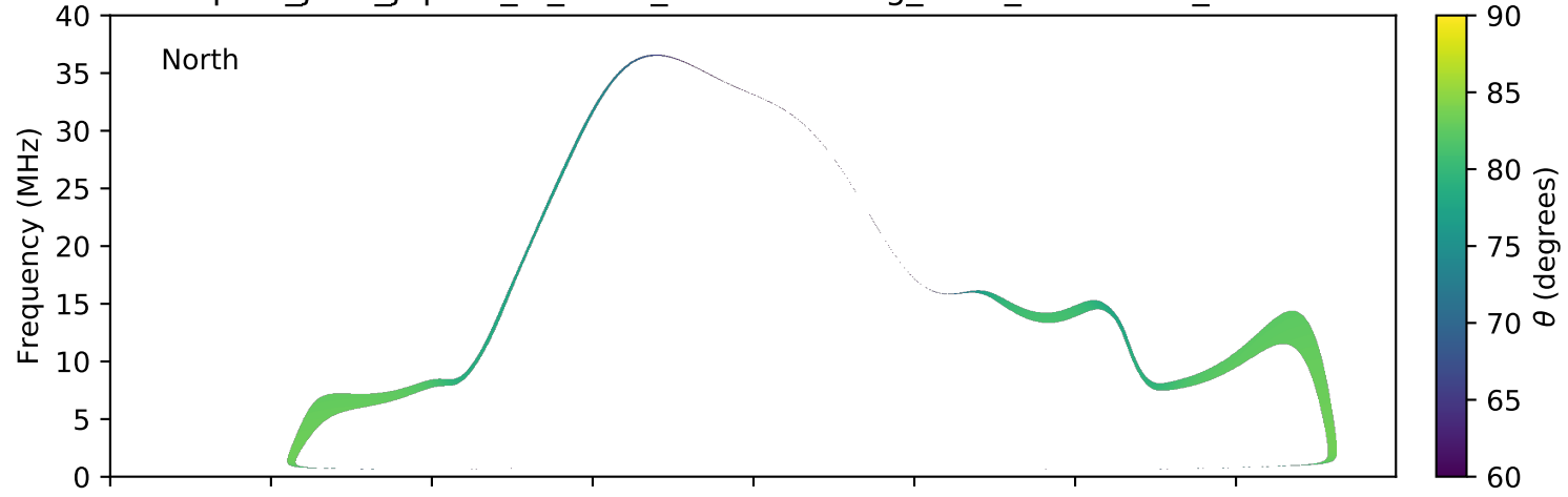
expres_juno_jupiter_io_isaac_lossc-wid1deg_3kev_20170418_v01.cdf
