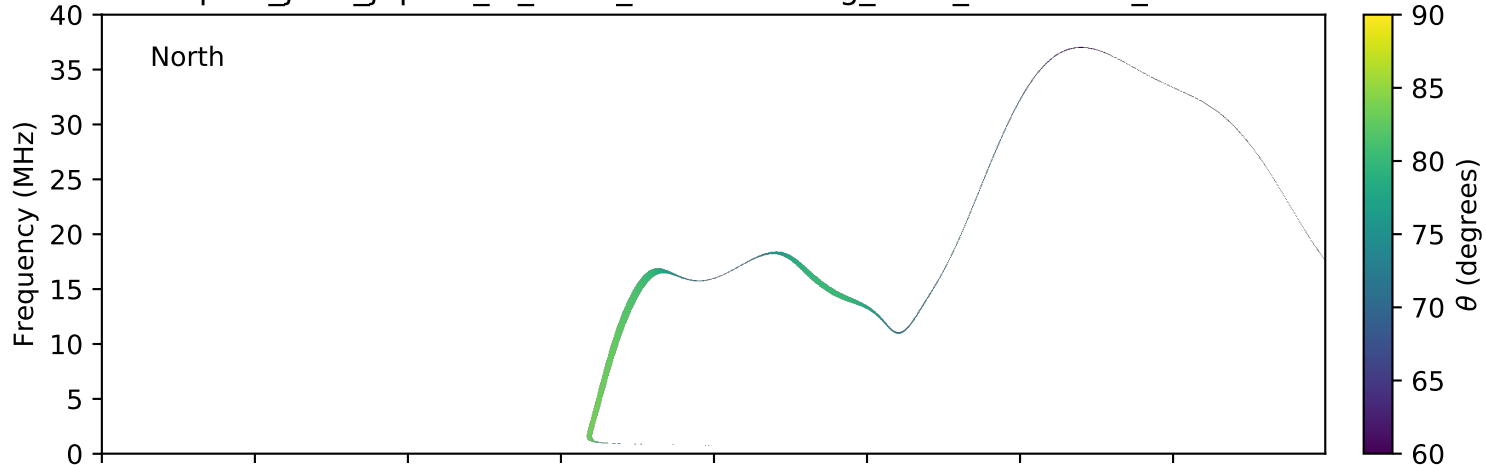
expres_juno_jupiter_io_isaac_lossc-wid1deg_3kev_20170416_v01.cdf
