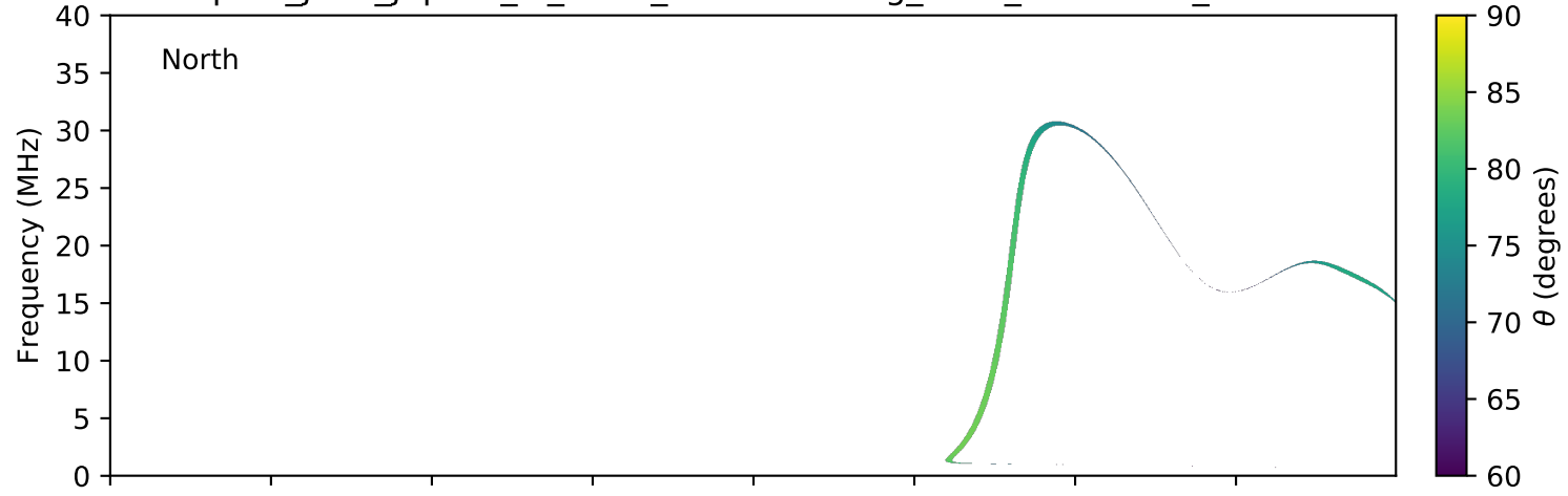
expres_juno_jupiter_io_isaac_lossc-wid1deg_3kev_20170414_v01.cdf
