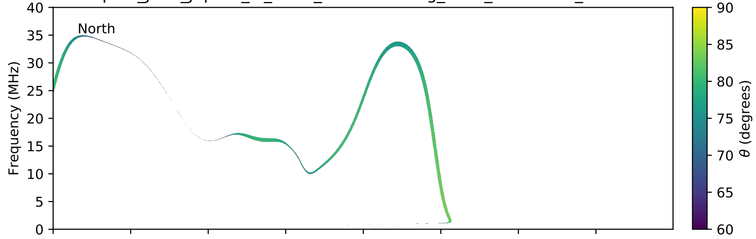
expres_juno_jupiter_io_isaac_lossc-wid1deg_3kev_20170413_v01.cdf
