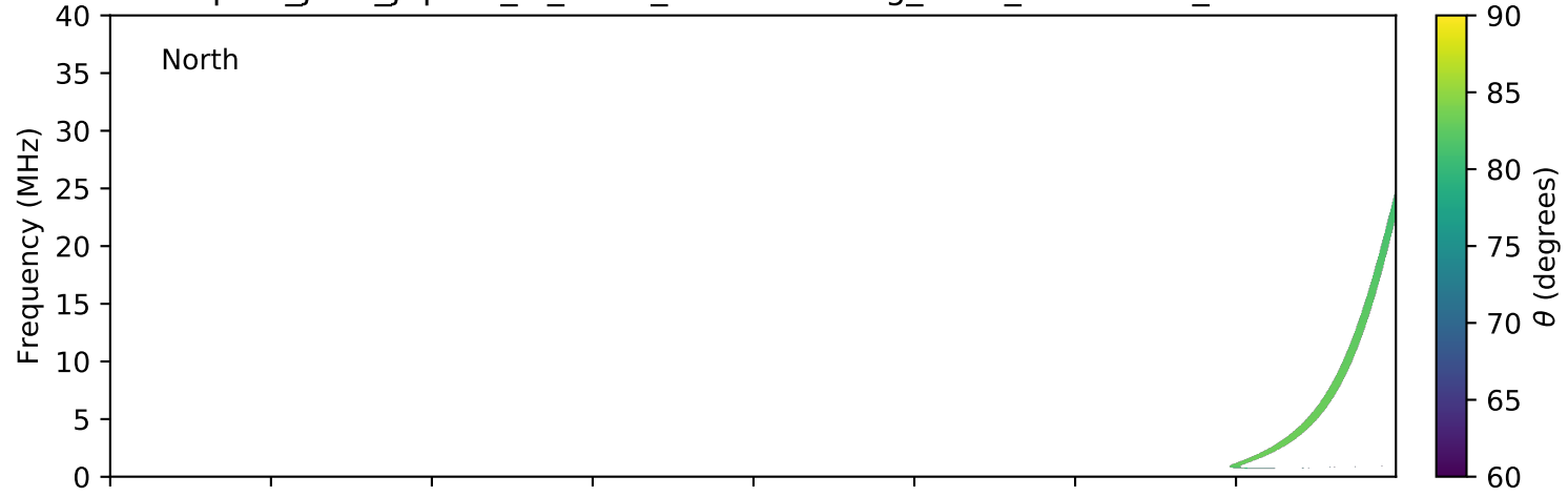
expres_juno_jupiter_io_isaac_lossc-wid1deg_3kev_20170412_v01.cdf
