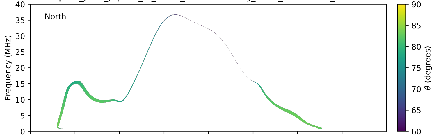
expres_juno_jupiter_io_isaac_lossc-wid1deg_3kev_20170411_v01.cdf
