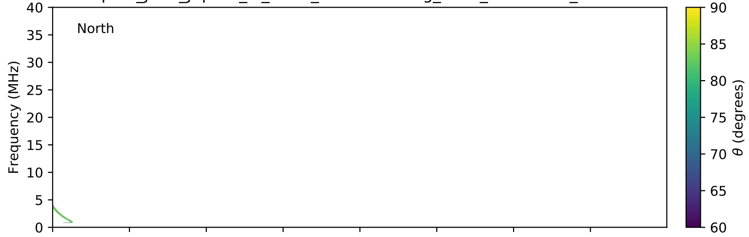
expres_juno_jupiter_io_isaac_lossc-wid1deg_3kev_20170410_v01.cdf
