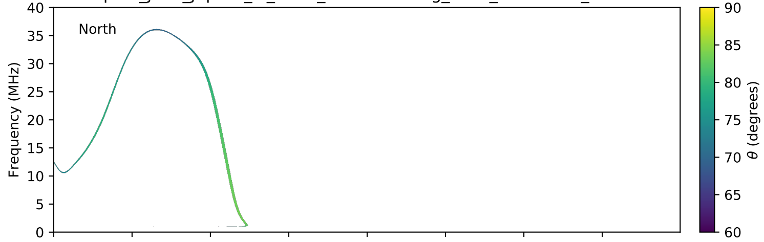
expres_juno_jupiter_io_isaac_lossc-wid1deg_3kev_20170408_v01.cdf
