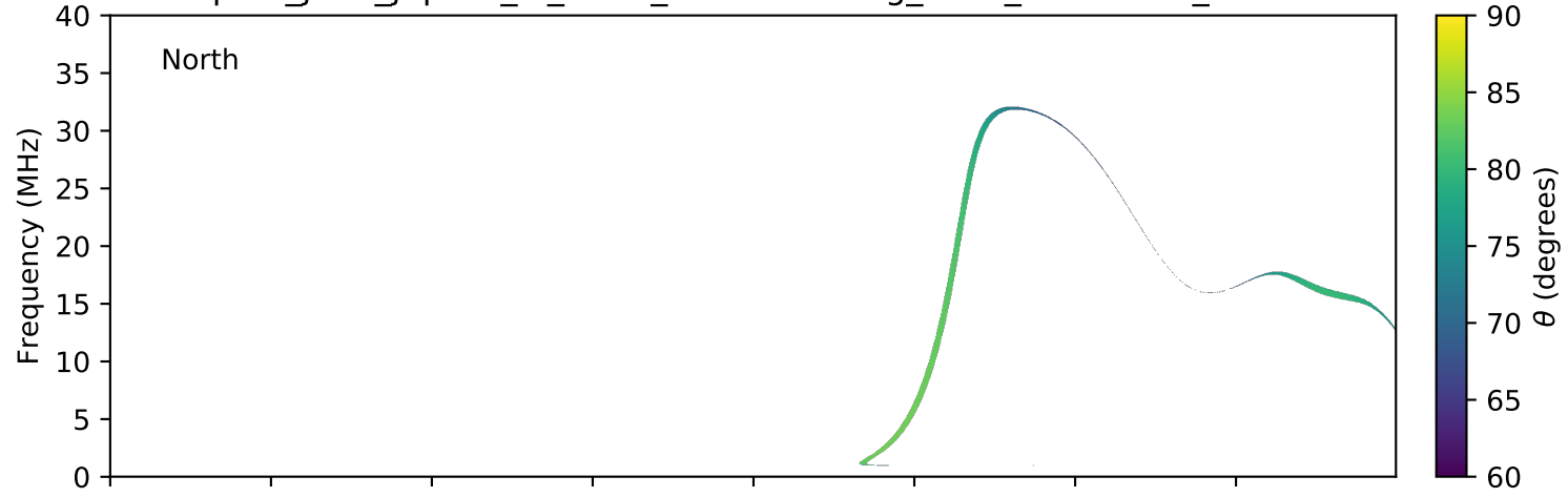
expres_juno_jupiter_io_isaac_lossc-wid1deg_3kev_20170407_v01.cdf
